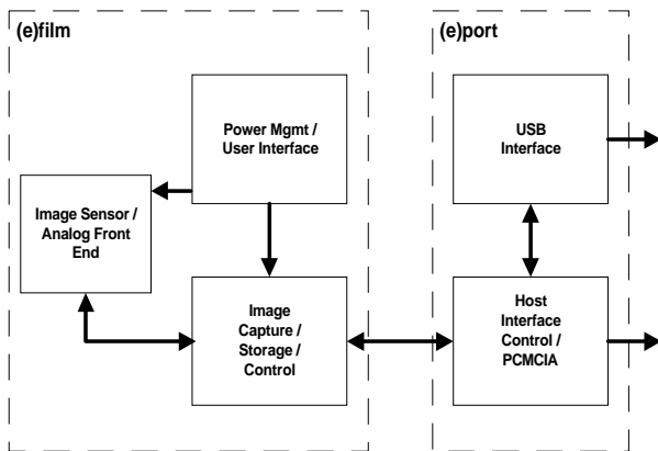
Figure 2. Functional Block Diagram of (e)film and (e)port
